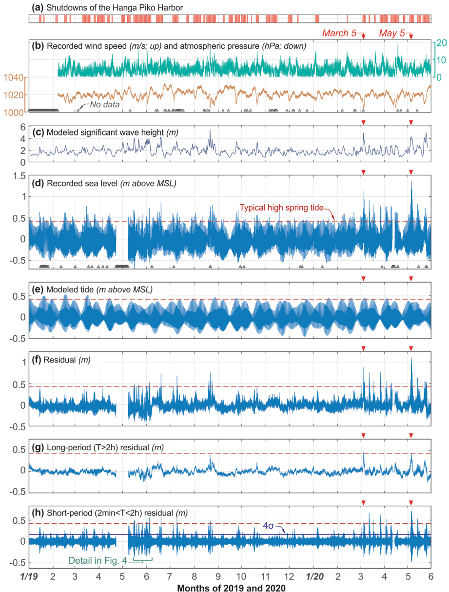
Fig. 3 Main datasets time series used in this study. a Shutdowns of the Hanga Piko Harbor (red lines). b Recorded wind speed (green) and atmospheric pressure (orange) at Mataverí Airport (See Fig. 1b for station location). c Modeled significant wave height at a node located 300 m off Hanga Piko at 20 m water depths (see Fig. 1b for node location). d Recorded sea level at Hanga Piko's tide gauge. e Modeled astronomical tide. f Residual sea level. g–h Long- and short-period component of the residual sea level, respectively. Blue horizontal line in (h) indicates four standard deviations ( 4\sigma ) from the mean, used as a threshold for meteotsunamis identification (Monserrat et al. 2006). All time series span from January 1st, 2019, to May 31st, 2020 (17 months). Red downward triangles indicate the March 5th and May 5th, 2020, extreme sea-level events analyzed in this study. The upward black triangles in b and d indicate positions of data gaps
