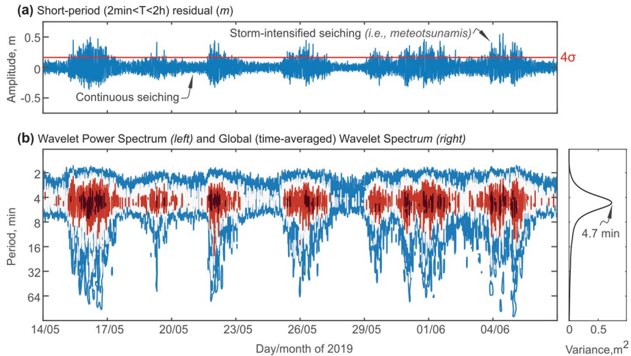
Fig. 4 Continuous and intensified seicheing. a A 24-day-long segment of the short-period component of residual sea level, between May 14 and June 7, 2019. Red horizontal line indicates four standard deviations ( 4\sigma ) from the long-term mean shown in Fig. 3h. According to Monserrat et al. (2006), amplitudes exceeding this threshold are defined as meteotsunamis. b Wavelet power spectrum (left) and normalized global wavelet spectrum (right) for the time series in (a). Reddish colors indicate large energy levels, and bluish colors indicate lower energy levels
